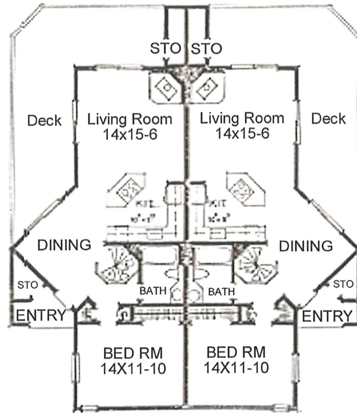
FIRST FLOOR 714 sq. ft per unit
